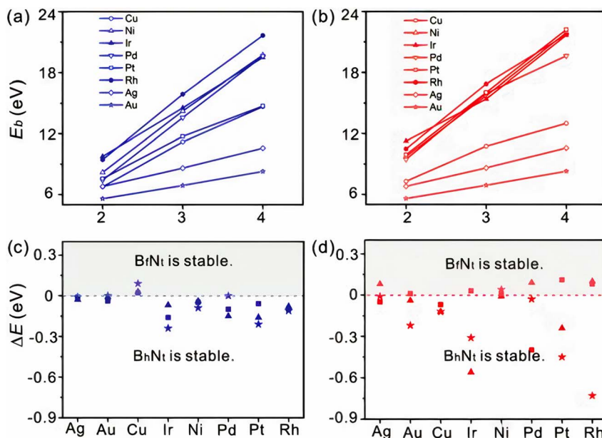
Fig. 3 Binding energies as a function of BN clusters terminated with (a) N and (b) B atoms. The difference in formation energy between B_rN_t and B_hN_t of (c) N and (d) B terminated BN clusters. Squares, stars, and triangles represent the cluster size of 2, 3, and 4, respectively. 180
