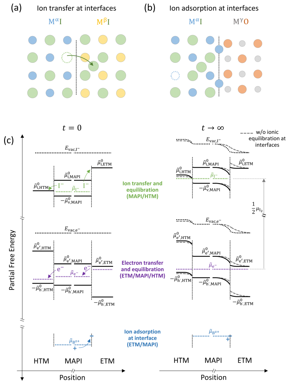
Fig. 7 (a) Ionic equilibration between two metal iodide phases M^{\alpha}I and M^{\beta}I , where transfer of I^{-} from M^{\alpha}I to M^{\beta}I increases the concentration of V_{I}^{\bullet} on the left side and of I_{I}^{\prime} on the right side of the interface giving rise to an interfacial equilibrium space charge ( \Delta\mu_{I^{-}} \neq 0 and different standard potentials of defect formations in the two phases are assumed). (b) Metal cation adsorption from a metal iodide M^{\alpha}I on the interface of a second phase (here an oxide M^{\gamma}O ) induces a space charge region where positive defects are depleted and the concentration of negative defects (here V_{M}^{\bullet} and I_{I}^{\prime} ) is increased. (c) Example of an extended ionic and electronic energy diagram of a MAPI solar cell in the dark at equilibrium where the interfaces are highlighted. Ion transfer (here I^{-} ) and ion adsorption (here B^{z+} adsorbed at the MAPI/ETM interface, e.g. Pb^{2+} adsorbed on TiO_2 surface 47 ) can have significant repercussion on the chemical and electrostatic situation at interfaces. The situations upon contact ( t = 0 ) and after equilibration ( t \rightarrow \infty ) are shown. In the right diagram, dashed lines indicate the situation where ionic equilibration with contact materials is not considered.
