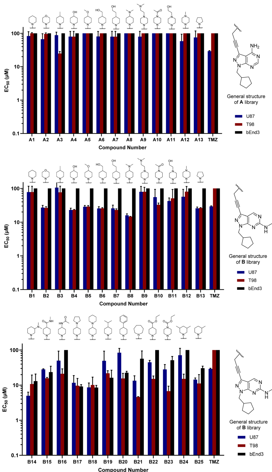
Fig. 2 Cell screening of initial libraries A and B. EC_{50} values calculated for A1-13 (top), B1-13 (middle) and B14-25 (bottom), and positive control TMZ against U87, T98 and bEnd3 cells. Data obtained from a cell viability assay where PrestoBlue® reagent was added after drug treatment for 5 d at 30, 10 and 3 \mu M doses. Error bars: \pm SD from n = 3 .
