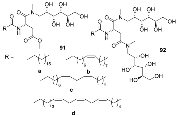
Fig. 58 Glycolipid containing unsaturated tail.
