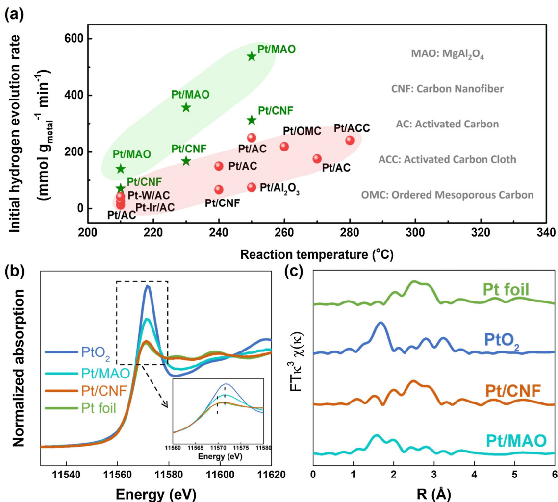
Fig. 2 (a) Comparison of dehydrogenation activity of Pt/MgAl 2 O 4 and Pt/CNF with other catalysts at different temperatures. (b) Normalized Pt L 3 -edge XANES spectra and (c) k 3 -weighted Fourier transform EXAFS spectra (L 3 -edge) of Pt for Pt foil, PtO 2 , Pt/CNF, and Pt/MgAl 2 O 4 . 91 Modified with permission from ref. 91. Copyright (2021) Elsevier Inc.
