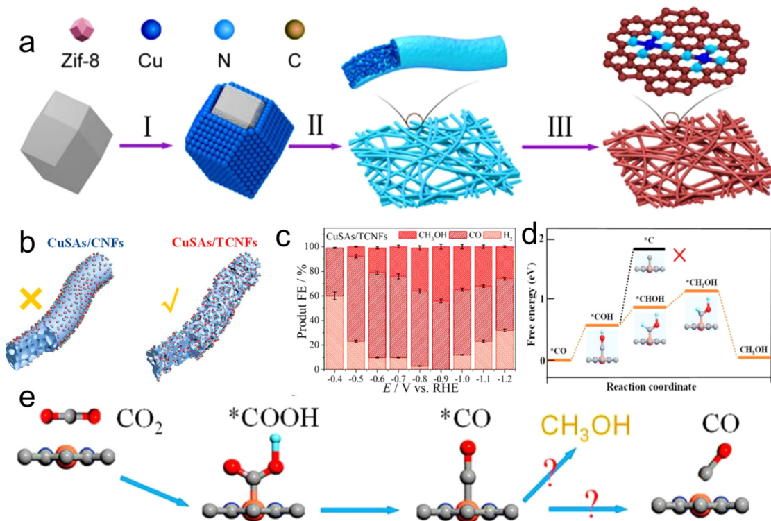
Fig. 22 (a) Synthesis of Cu single atom. (b) Illustration of \text{CO}_2 diffusion on two samples. (c) FEs of products. (d) Free energy model for the conversion of \text{*CO} to methanol. (e) Optimized atomic structures of CuSAs/TCNFs and proposed reaction paths for \text{CO}_2 electroreduction. Reproduced with permission from ref. 206 Copyright 2019, ACS.
