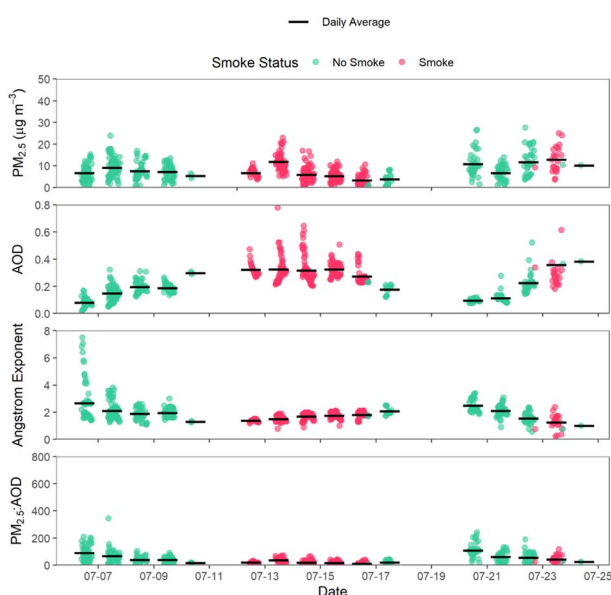
Fig. 6 Time-series plots of PM_{2.5} , AOD, Angstrom exponent, and PM_{2.5} :AOD ratio from July 6, 2021, to July 24, 2021, from four CEAMS sites in Southern California, colored by HMS-derived smoke status. Measurements are from four AMODv2s (Fig. 1). Note that measurements on July 12, 2021, were from a single AMODv2 started early by the CEAMS participant.
