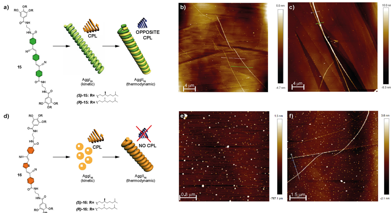
Fig. 8 Chemical structures of compounds 15 (a) and 16 (d) and schematic representation showing the CPL-emitting kinetic and thermodynamically controlled aggregated structures formed by 15 and 16 . AFM images of the kinetically controlled AggI 15 (b), thermodynamically controlled AggII 15 (c) kinetically controlled AggI 16 (e) and thermodynamically controlled AggII 16 (f) (MCH/CHCl 3 9/1 as the solvent; HOPG as the surface; c_T = 10 mM) (reproduced from ref. 66 with permission from the Royal Society of Chemistry, copyright 2022).
