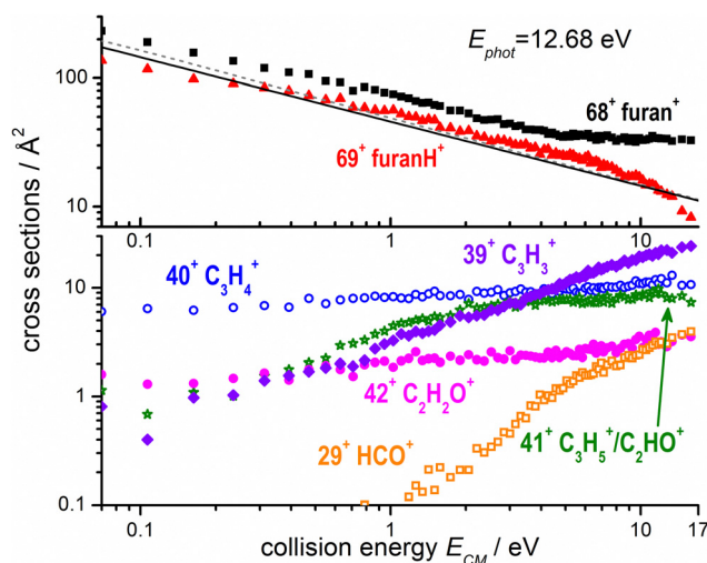
Fig. 3 Absolute reactive cross sections (in log scale) for products ( m/z = 69, 68 , top panel; m/z = 42, 41, 40, 39 and 29 bottom panel) measured as a function of the collision energy ( E_{\text{CM}} ) from ion–molecule collision of \text{H}_2\text{O}^{+\bullet} with furan, with \text{H}_2\text{O}^{+\bullet} produced by direct photoionization at h\nu = 12.68 eV. The black line is the Langevin capture cross section calculated using a value of 7.3 \text{ \AA}^3 for the averaged polarizability of furan, 61 while the grey dashed line was calculated also taking into account the dipole moment of furan ( \sim 0.7 Debye). 62 Estimated uncertainties on the absolute values of the CSs are about 20%. Error bars are not shown for the sake of clarity.
