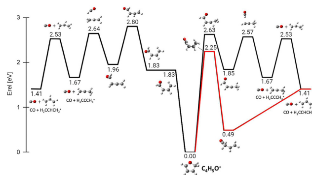
Fig. 13 ZPV-corrected relative energy diagram corresponding to the CO loss channels (fragment 41^+ ) from the protonated isomer 2 of furan. Relative energies with respect to isomer 2 (in eV) obtained at the B3LYP/6-311++G(d,p) level of theory, including the ZPE correction, are indicated for each structure and TS. In red the lowest energy pathway with the concerted ring opening and H shift from C5 to C4.
