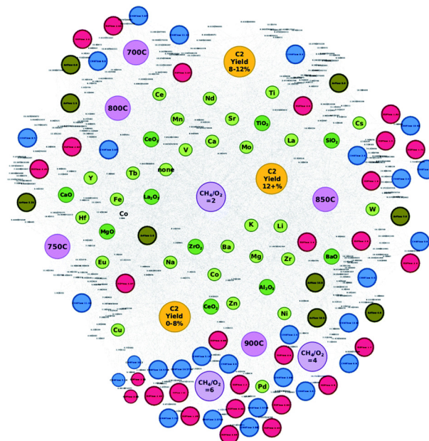
Fig. 13 Catalyst network using oxidative coupling of methane catalysts big data. The relationships between C 2 yield and composition and experimental conditions are unveiled. Reproduced from ref. 32 with permission from the Royal Society of Chemistry.
