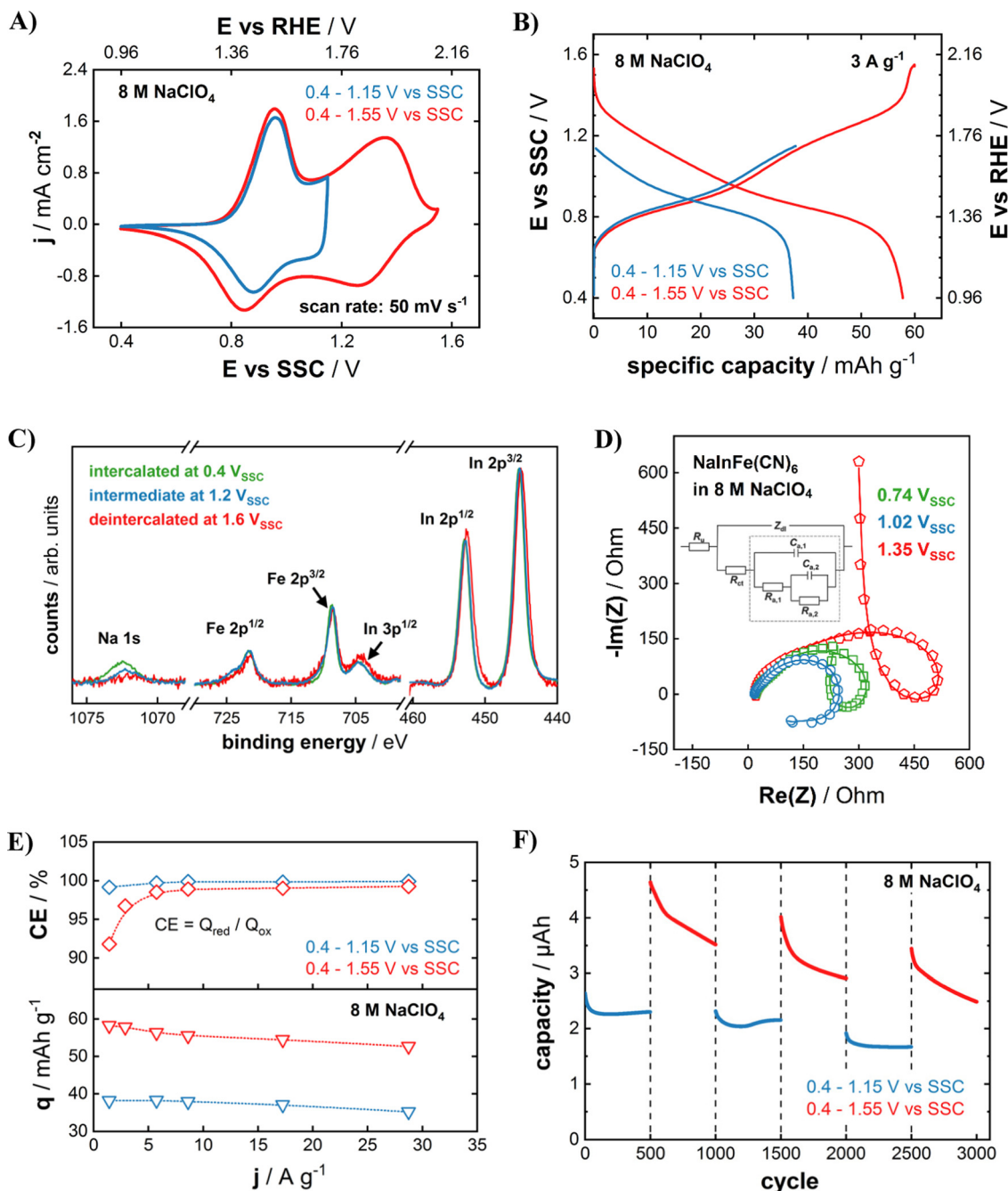
Fig. 3 Impact of the anodic cut-off potential on electrochemical performance. (A) CVs and (B) galvanostatic charge–discharge curves for InHCF in 8 M NaClO _4 for E_{\text{cut-off}} = 1.15 \text{ V} (blue curves) and 1.55 \text{ V} (red curves) vs. SSC. For a better correlation to the electrolyte stability window, the potentials are also given with respect to the RHE scale (pH = 5.8 for 8 M NaClO _4 ). (C) XPS analysis of InHCF films in three different states of charge (cut-off potentials of 0.4 V, 1.2 V and 1.6 V vs. SSC). (D) EIS spectra of InHCF electrodes in 8 M NaClO _4 at three different potentials (0.74 V, 1.02 V and 1.35 V vs. SSC). Open symbols are the obtained spectra and lines are the resulting fits. The inset figure represents the used equivalent circuit diagram for fitting the collected impedance spectra (see main text). (E) Obtained specific capacity q and Coulombic efficiency CE for different (dis)charging currents in galvanostatic cycling, as well as (F) cycling stability for the lower and higher E_{\text{cut-off}} . The dotted red and blue lines in (E) serve as a guide to the eye.
