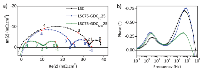
Fig. 4 (a) Nyquist plot of normalized EIS spectra and (b) bode-phase plot for LSC, LSC75-GDC CC 25 and LSC75-GD MW 25 cathodes at 700 °C under synthetic air flow. Inserted numbers close to red data points are their log(frequency) value. In (a), the pure resistive contribution of the electrolyte was subtracted from the data for easy comparison.
