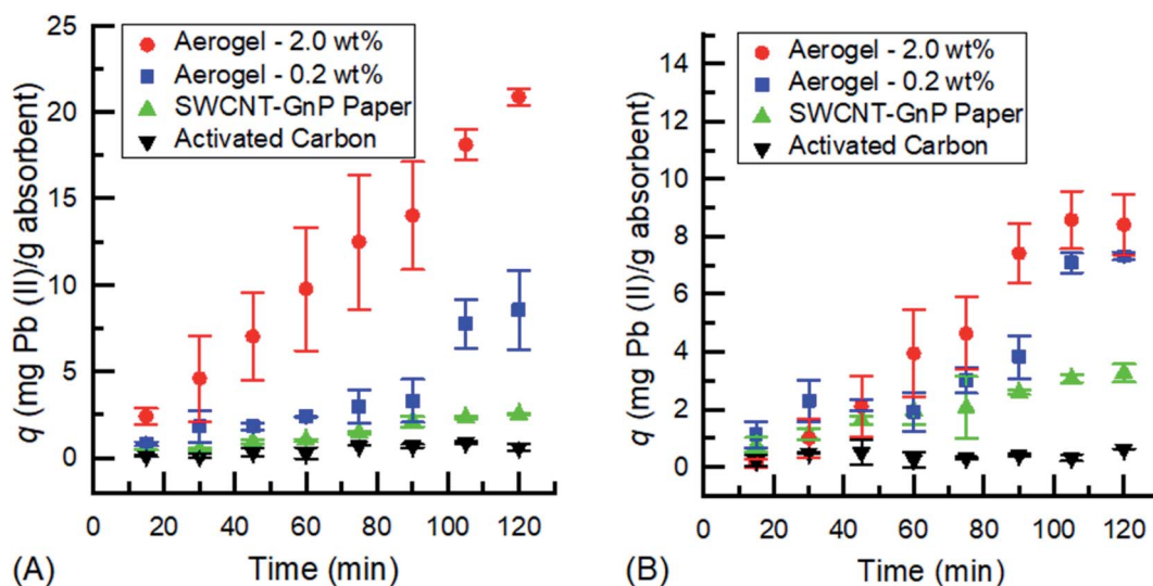
Fig. 5 Time dependent adsorption for removal of adsorbate ( \text{Pb(II)} ) with initial concentrations of (A) 0.5 \text{ mg mL}^{-1} and (B) 0.1 \text{ mg mL}^{-1} by carbon nanomaterial (CNM)-based aerogels of (●) 2.0 wt% and (■) 0.2 wt%, (▲) SWCNT-GnP hybrid paper, and (▼) activated carbon.
