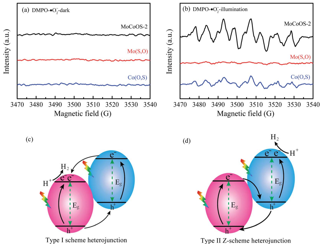
Fig. 14 EPR spectra of (a) \text{DMPO}-\cdot\text{O}_2^- and (b) \text{DMPO}-\cdot\text{O}_2^- for \text{Mo}(\text{S},\text{O}) , \text{Co}(\text{O},\text{S}) , and \text{MoCoOS} catalysts under darkness and illumination for 10 min. (c and d) The two types of heterojunction.
