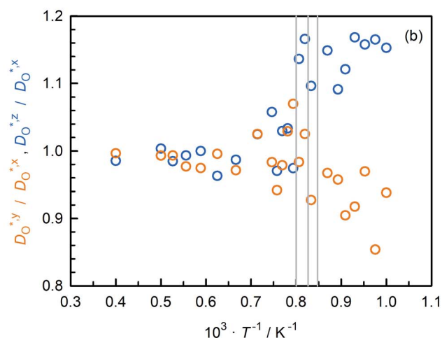
Fig. 4 Oxygen tracer diffusion coefficients obtained for a \text{CaTiO}_3 system containing only oxygen vacancies as a function of inverse temperature: (a) total values, (b) ratios of axis-specific values. Error bars are smaller than the symbol size.
