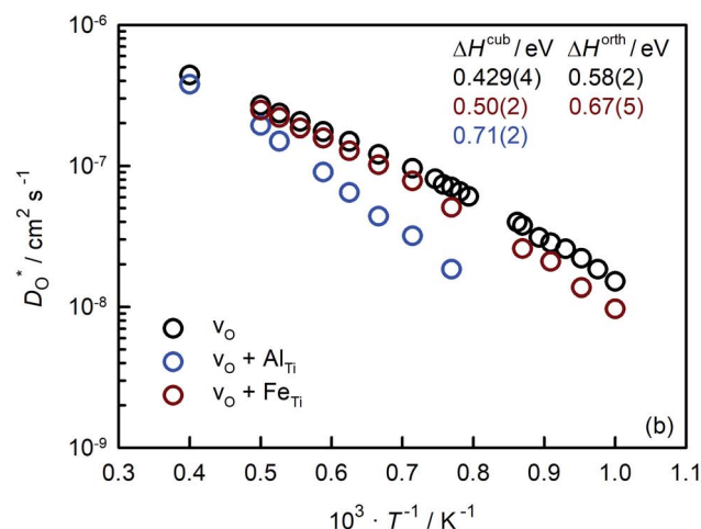
Fig. 5 Tracer diffusion coefficients of oxygen obtained for \text{CaTiO}_3 with oxygen vacancies and charge-compensating acceptor-type defects: (a) native acceptor defects, (b) foreign acceptor defects. In all cases, the site fraction of oxygen vacancies was n_v = 0.2\% .
