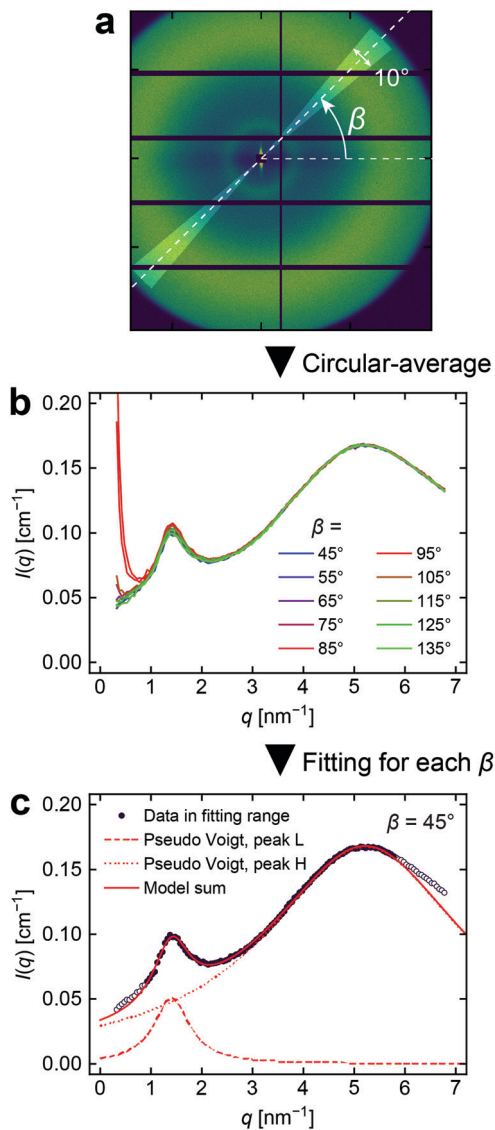
Fig. 5 Procedure for the SAXS data analysis. (a) Example of the region used for sector averaging. The case of \beta = 45^\circ for B at \lambda = 1.83 is shown as an example. (b) 1D profiles at each \beta indicated, obtained by sector averaging the image in Panel a. (c) Representative example of the curve fitting for 1D profiles. The symbols are the data at \beta = 45^\circ in Panel b. The data points used for the fitting are indicated by closed symbols. Dotted, dashed, and solid curves represent two pseudo Voigt functions and their sum used for fitting, respectively.
