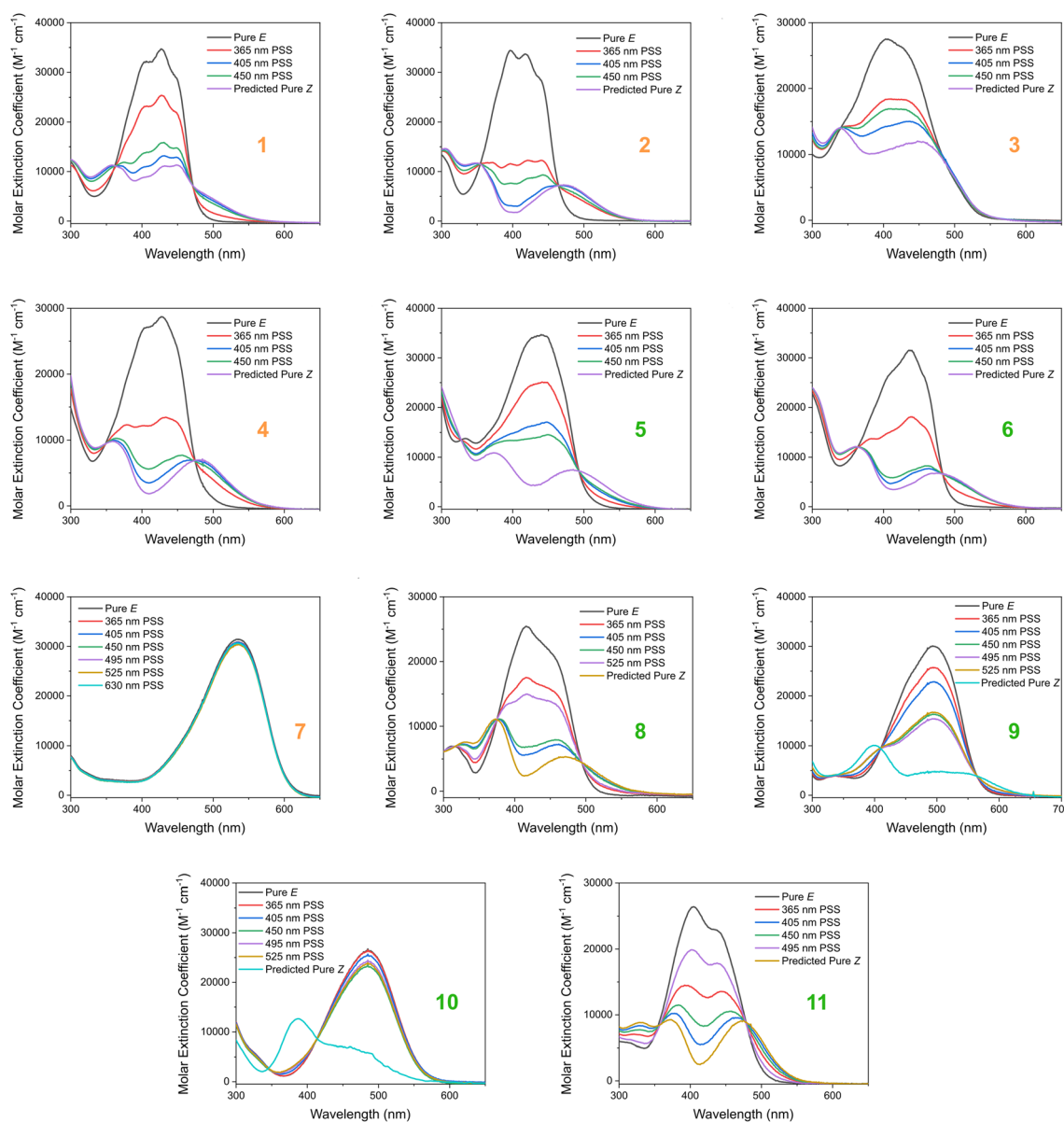
Fig. 5 The experimental UV-vis absorption spectrum of switches 1–11 measured at 25 \mu M in DMSO and shown as the molar extinction coefficient ( M^{-1} \text{ cm}^{-1} ). Different irradiation wavelengths were employed in order to predict the “pure” Z spectra using the procedure detailed by Fischer. 81 The chemical structures of these switches are shown in Fig. 4 above.
