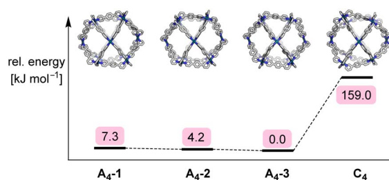
Fig. 5 Schematic of the relative energy differences of the four isomers A4-1 , A4-2 , A4-3 , and C4 of complex [\text{Pd}_{12}(\text{L1})_{24}]^{24+} , along with graphics of the HSE06/Def2-SVP-optimized structures.
