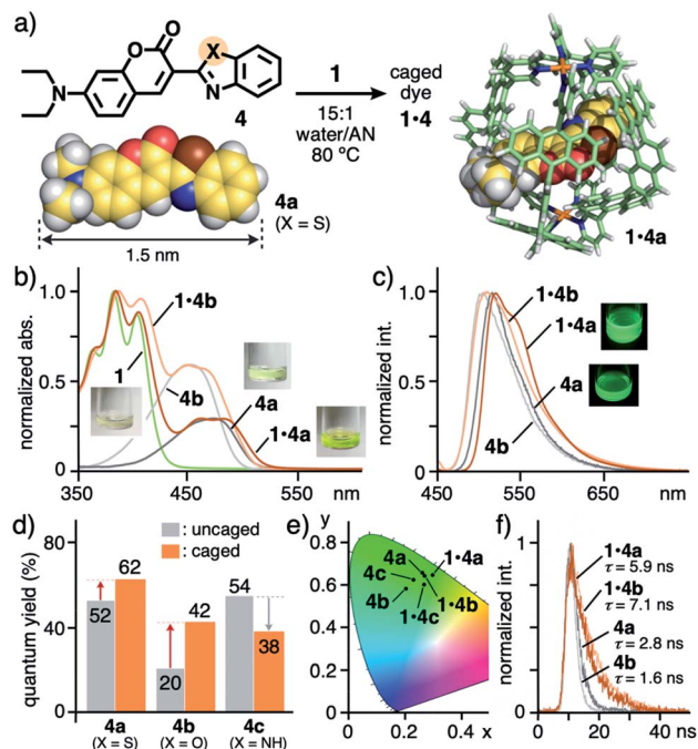
Fig. 3 (a) Formation of caged dyes 1·4 ( X = S, O , and NH ) and the optimized structures of 4a and 1·4a ( R^1 = H for clarity). 11 (b) UV-visible spectra and photographs (r.t., 15 : 1 water/acetonitrile (AN)) of 1·4a , 1·4b , 1 , and 4a , 4b (in 2 : 1 water/AN), (c) their fluorescence spectra ( \lambda_{\text{ex}} = 450 nm) and (d) quantum yields, and (e) their CIE diagram (before and after binding by 1 ). (f) Fluorescence lifetimes (r.t., \lambda_{\text{ex}} = 355 nm, 15 : 1 or 2 : 1 water/AN) of 1·4a , 1·4b , and 4a , 4b .
