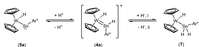
Scheme 6 Addition and abstraction of protons and hydride ligands. (i): rt, LiAlH 4 , Et 2 O; (ii): rt, [Ph 3 C][Al(OC{CF 3 }) 4 ], o-DFB.
