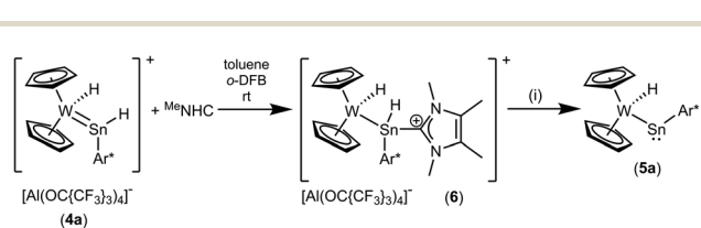
Scheme 5 (i): Toluene/o-DFB, 80 °C, 3d, – [ Me NHC–H][Al(OC{CF 3 }) 4 ].
