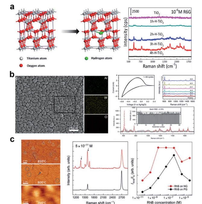
Fig. 2 Doped semiconductor substrates and SERS activity. (a) Crystal structure of \text{TiO}_2 and hydrogenated \text{TiO}_2 and Raman spectra of R6G on \text{TiO}_2 with different levels of hydrogenation. Reproduced with permission from ref. 42. Copyright 2018, American Chemical Society. (b) EDX analysis of Al-intercalated \text{WO}_3 and its SERS performance characterization. Reproduced with permission with ref. 43. Copyright 2019, Springer Nature. (c) STM images of N-doped graphene under different synthesis conditions and SERS performance characterization. Reproduced with permission from ref. 61. Copyright 2016, AAAS.
