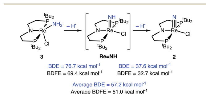
Scheme 6 DFT (B3LYP/def2-TZVP) computed thermochemistry for the oxidation of 3 to 2 via stepwise H-atom removal.
