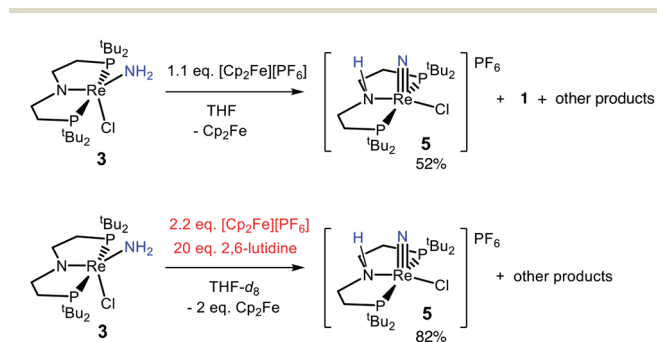
Scheme 5 Reactions of 3 with chemical oxidants.
