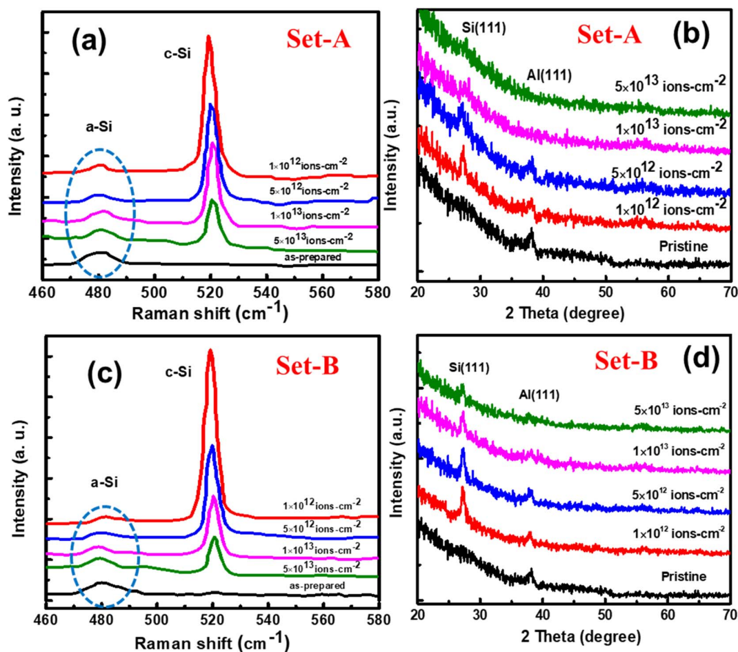
Fig. 4 (a) Raman spectra (b) XRD pattern of set-A irradiated by 100 MeV Ni ions at 100 °C with different fluence of 1 \times 10^{12} ions per cm 2 , 5 \times 10^{12} ions per cm 2 , 1 \times 10^{13} ions per cm 2 , and 5 \times 10^{13} ions per cm 2 . And (c) Raman spectra (d) XRD of set-B irradiated at 100 °C with different fluences at 100 °C with different fluence of 1 \times 10^{12} ions per cm 2 , 5 \times 10^{12} ions per cm 2 , 1 \times 10^{13} ions per cm 2 , and 5 \times 10^{13} ions per cm 2 . [Reproduced/adapted from Maity et al. , 157 RSC Adv. , 2020, 10, 4414, with permission from The Royal Society of Chemistry.]
