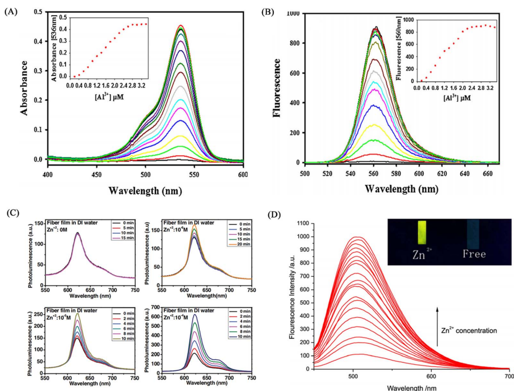
Fig. 18 Sensing properties of Zn 2+ , Al 3+ sensor. (A) and (B) reprinted with permission from ref. 122. Copyright 2016, Elsevier. (C) Reprinted with permission from ref. 123. Copyright 2013, Wiley-VCH (D) reprinted with permission from ref. 124. Copyright 2017, Chen Zhou et al.
