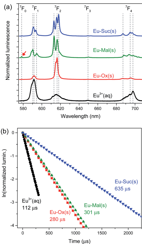
Fig. 3 Luminescence from {}^5\text{D}_0 \rightarrow {}^7\text{F}_J ( J = 0-4 ) transitions of solid Eu–Ox, Eu–Mal, and Eu–Suc compounds: (a) luminescence spectra and (b) luminescence decay plots. The samples were the same as those used for the powder XRD measurements. The red arrow indicates {}^5\text{D}_0 \rightarrow {}^7\text{F}_0 transition peak in the Eu–Mal luminescence.
