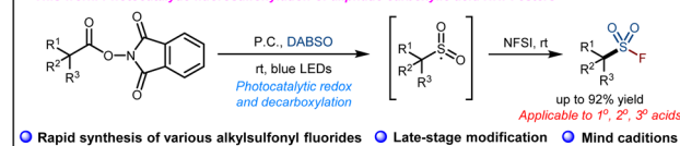
Scheme 1 Approaches for fluorosulfonyl group installation via SO 2 radical insertion/fluorination.
