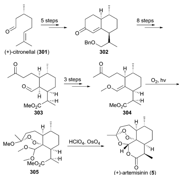
Scheme 29 Total synthesis of (+)-artemisinin by Zhou.
