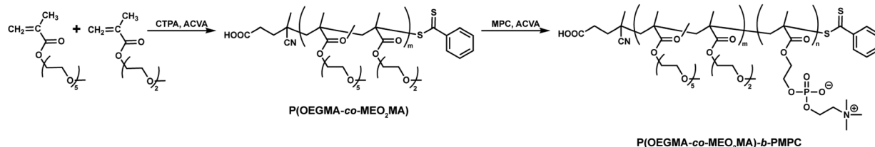
Scheme 1 Synthesis of P(OEGMA- co -MEO 2 MA)- b -PMPC.
