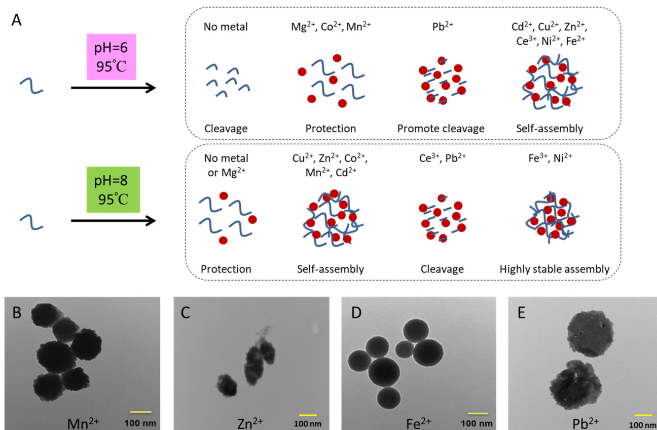
Fig. 2 (A) Classification of the effects of metal ions by incubating them with the DNA at 95 °C for 3 h at pH 6 and pH 8. TEM micrographs of nanoparticles formed by the 24-mer DNA and (B) Mn 2+ , (C) Zn 2+ , (D) Fe 2+ , and (E) Pb 2+ . The Fe 2+ NPs were prepared in water and the rest were prepared in 5 mM MOPS buffer at pH 8.
