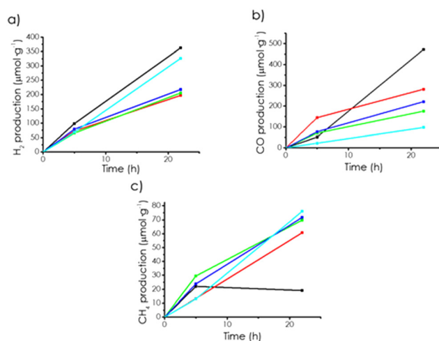
Fig. 4 Temporal profiles of (a) H _2 , (b) CO, and (c) CH _4 evolution for mp-C _{\alpha} (black), mp-C _{\beta} (red), mp-C _{\gamma} (green), mp(N)-C _{\alpha} (blue), and mp(P)-C _{\alpha} (cyan) upon the irradiation of CO _2 dissolved in CH _3 CN/H _2 O containing TEOA with the output of a 300 W Xe lamp.
