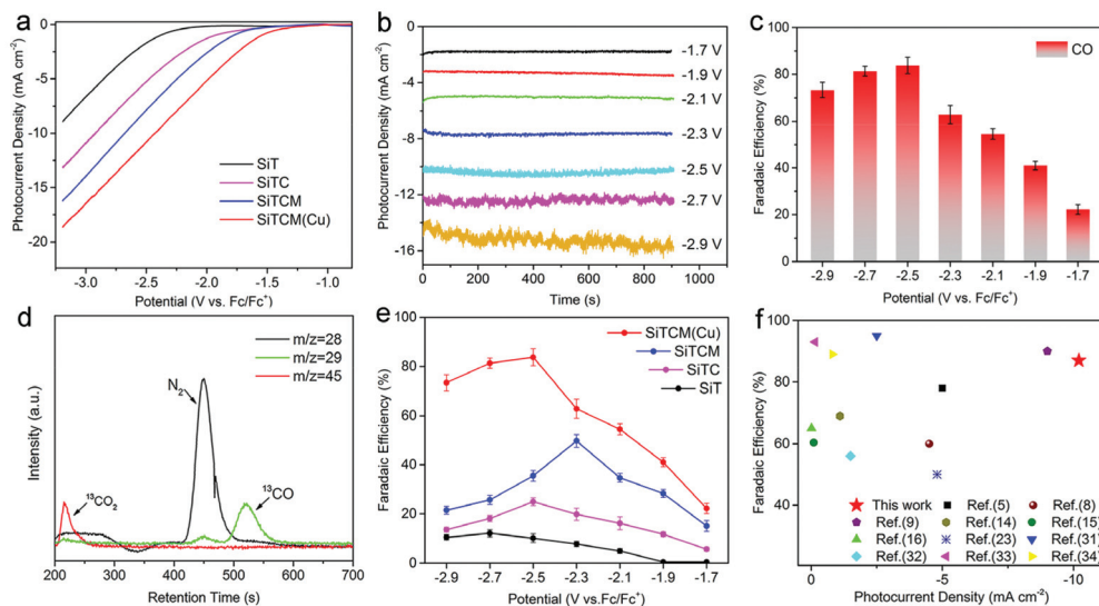
Fig. 3 PEC CO 2 R performance of SiTCM(Cu). (a) Comparison of LSVs for SiT, SiTC, SiTCM and SiTCM(Cu) under illumination. (b) Chronoamperometric i-t curves and (c) CO faradaic efficiencies of SiTCM(Cu) at various potentials. (d) GC-MS spectra of the isotopic 13 CO 2 test on SiTCM(Cu). (e) Comparison of the CO faradaic efficiency of SiT, SiTC, SiTCM and SiTCM(Cu) at various potentials. (f) Comparison of the CO 2 RR FE and photocurrent density from this study with recent literature engaging state-of-the-art PEC catalysts (see Table S1† for reference details).
