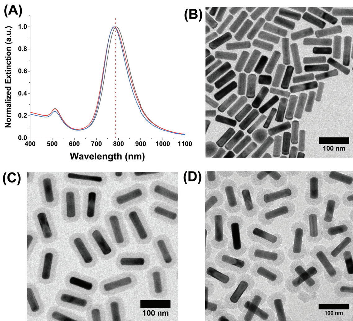
Fig. 2 (A) UV-Vis-NIR extinction spectra of the CTAB-coated gold nanorods in water (black), full-shell silica-coated gold nanorods (red), and end-shell silica-coated gold nanorods (blue) in ethanol. The dashed line denotes 785 nm (the laser excitation wavelength). TEM micrographs of the (B) CTAB coated, (C) AuNR@Full, and (D) AuNR@End rods, respectively. All scale bars are 100 nm.
