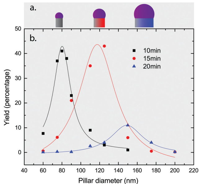
Fig. 3 (a) Schematics showing the increase in droplet volume with \text{SiO}_2/\text{Si} pillar diameter at a fixed contact angle. (b) Vertical yield as a function of \text{SiO}_2/\text{Si} pillar nominal diameter for Ga predeposition times of 10 min, 15 min and 20 min.
