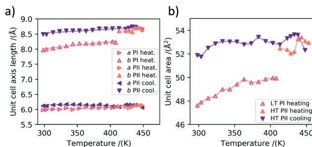
Fig. 5 a) Lattice constants a and b during heating ( \blacktriangleright , \triangle ) and cooling ( \blacktriangleleft , \triangleright ). The filled triangles denote the high temperature polymorph II. It can be seen that the change in length is stronger for the b -axis in both polymorphs upon heating and cooling. b) The in-plane unit cell areas of both polymorphs plotted against the temperature. The filled in triangles denote polymorph II.
