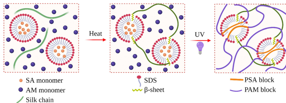
Fig. 14 Preparation of IPN hydrogels composed of SF and poly(acrylamide-co-styrene acrylate). Reproduced with permission from Wiley-VCH, copyright 2019. 163
