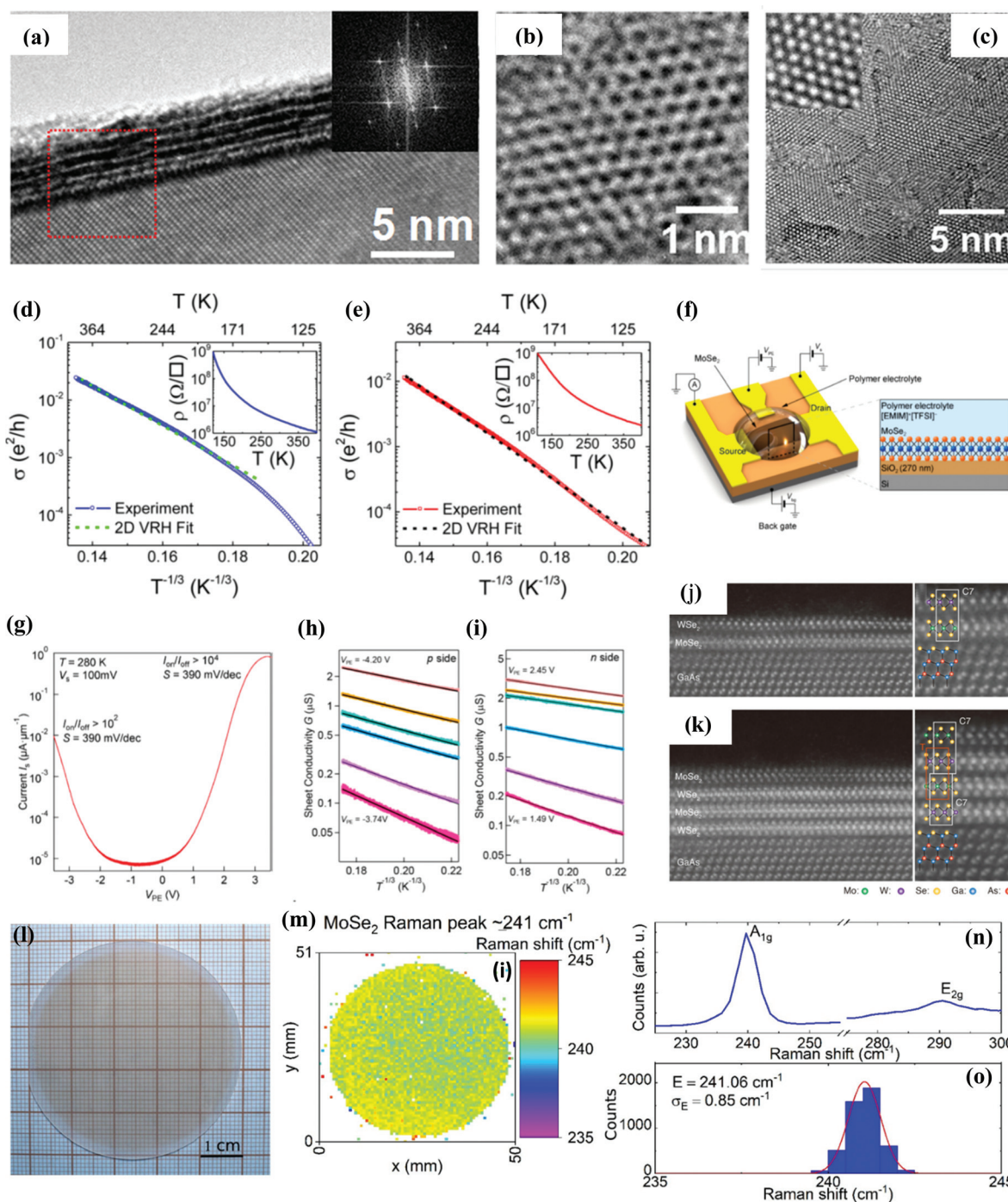
Fig. 3 (a) HR-STEM image of a layered structure of MoTe 2 . Inset shows the fast Fourier transform (FFT) of the area marked by the red square. The plan-view TEM image depicts the hexagonal arrangement of atoms in the (b) MoTe 2 thin film and (c) MoSe 2 lattice. Inset shows the zoomed-in view for 2 \times 2 \text{ nm}^2 . Electrical transport measurements show the conductivity variation with T^{-1/3} for (d) MoTe 2 and (e) MoSe 2 . Insets of (d, e) show the variations of the measured resistivities with temperature. The figures have been reproduced from ref. 67. (f) The schematic device structure of the MoSe 2 thin film-based EDLT. (g) Variation of the channel current with polymer electrolyte voltage (VPE) depicting ambipolar behavior. (h and i) Sheet conductivity ( G_{\text{SH}} ) as a function of T^{-1/3} on the p and n sides for different values of V_{\text{PE}} . The figure has been reproduced from ref. 45. The HAADF-STEM images for the (j) bilayered WSe 2 /MoSe 2 and (k) four-layered MoSe 2 /WSe 2 heterostructures grown on GaAs(111)B. The figure has been reproduced from ref. 71. (l) Optical image of epitaxially grown MoSe 2 . (m) Peak energy of the A 1g mode obtained through Raman mapping. (n) Typical Raman spectrum of MoSe 2 . (o) Distribution of the peak energy of the A 1g mode indicating the mean value and standard deviation. The figure has been reproduced from ref. 73.
