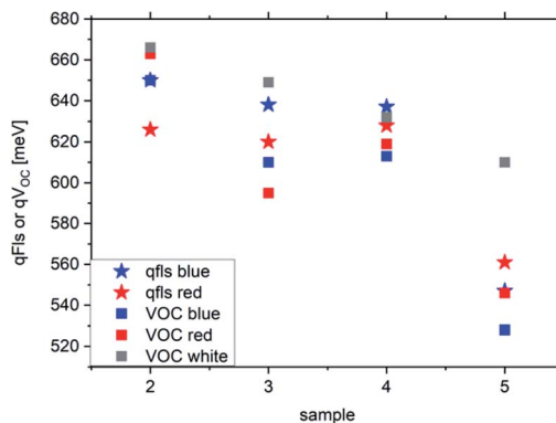
Fig. 7 qFls and V_{OC} for the \text{Cu(In,Ga)(S,Se)}_2 samples illuminated with a red laser (660 nm), a blue laser (405 nm) or a simulated AM1.5 spectrum (white).
