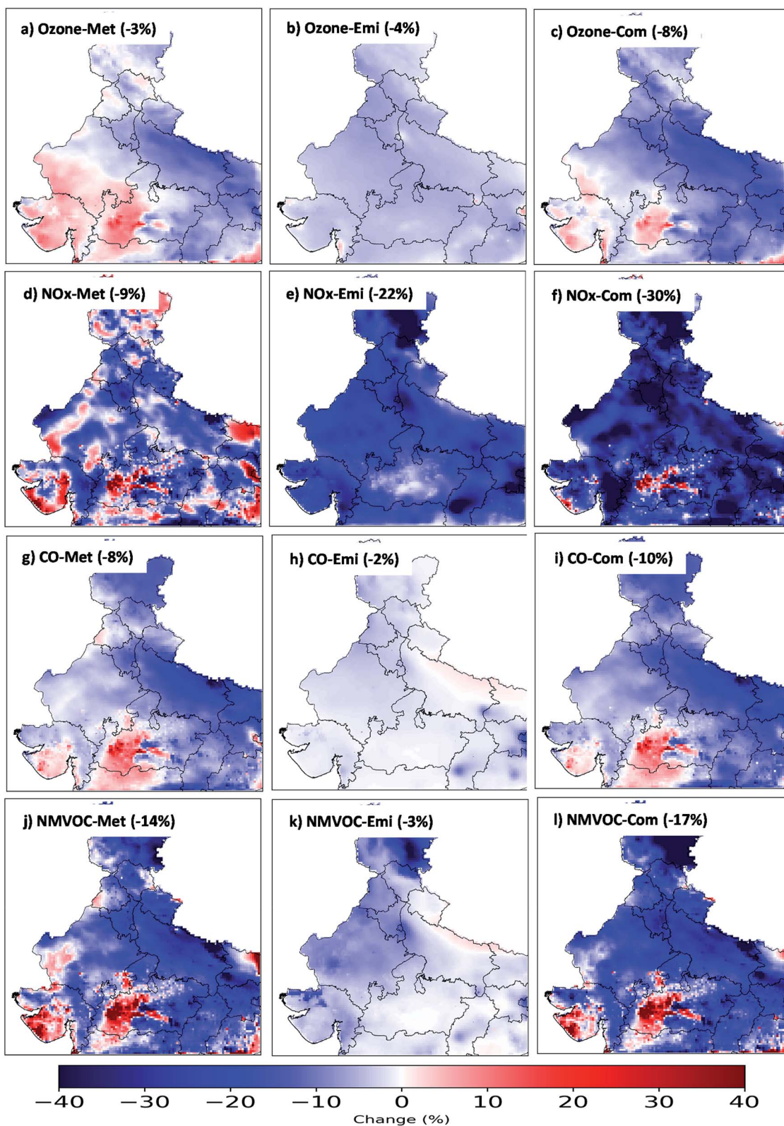
Fig. 8 Responses of April averaged daytime ozone (first row), NO x (second row), CO (third row), and NMVOC (fourth row) concentrations to meteorology (left column), emission (middle column), and combined (right column) effects. The numbers in parentheses show the averaged change over the colored region between April 2020 and 2019.
