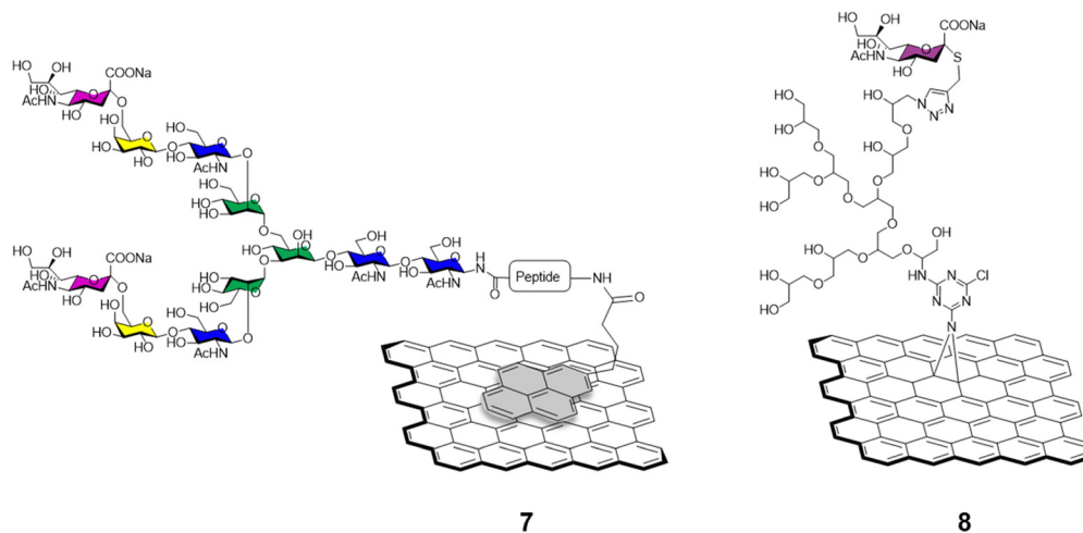
Fig. 3 Representative general structures of sialyglycopeptide-coated graphene via a pyrene (shown in light grey) 7 , and sialygraphene derivatives 8 which features trGO derivatives modified via a triazine moiety bearing a dendrimetic sialic acid conjugate.
