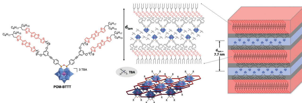
Fig. 20 Left: Molecular structure of the branched POM-BT TT hybrid oxocluster; middle: a schematic view of multi-layered self-assembly of the lamellar hybrid material, highlighting the specific arrangement of the POM/TBA double-layers (bottom, centre: showing POM clusters in blue and the surrounding TBA honeycomb structure in red – note the laterally offset bottom layer is shown in darker colours); Right: 3D schematic representation of lamellar nanomaterial, respecting the molecular segment sizes and shapes. This figure has been adapted from ref. 171 with permission from John Wiley and Sons, copyright 2021.
