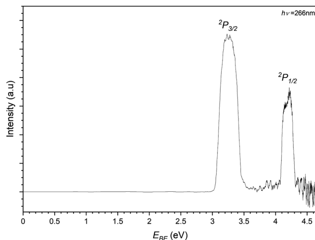
Fig. 8 Photoelectron spectrum of the 169 m/z peak from Fig. 3 assigned to photodetachment to the perturbed ^2P_{3/2} and ^2P_{1/2} states of the \text{I}^{\cdot\cdot}\cdots\text{C}_3\text{H}_6 complex.
