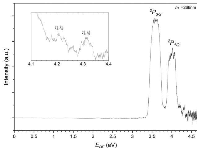
Fig. 6 Photoelectron spectrum of the 123 m/z peak from Fig. 2 assigned to photodetachment to the perturbed ^2P_{3/2} and ^2P_{1/2} states of the \text{Br}^{\cdot\cdot}\cdots\text{C}_3\text{H}_6 complex.
