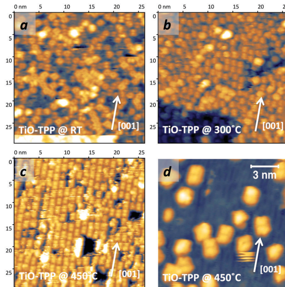
Fig. 23 STM images (W tip) of (a) 1 ML of TiO-TPP as deposited at RT, (b) after annealing to 300^\circ\text{C} and (c) 450^\circ\text{C} ; and (d) 0.2 ML of TiO-TPP after annealing to 450^\circ\text{C} .
