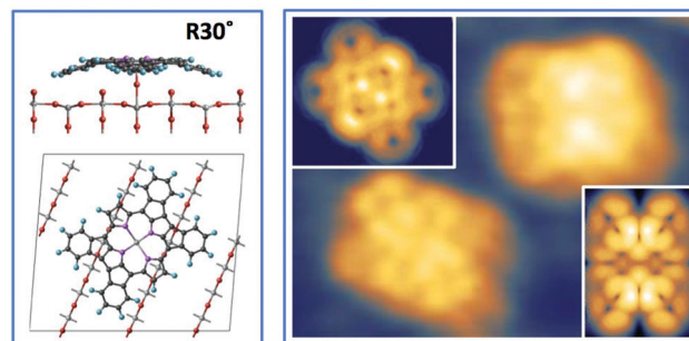
Fig. 25 Left: Side and top views of the equilibrium configuration of the most favoured \text{R}30^\circ orientation of the \text{TiO}^{\text{down-TPP-deH}} species atop a \text{Ti}_{5f} atom. Right: Close-up STM image of the two main types of flat TPP-deH molecules, \text{R}60^\circ and \text{R}0^\circ on \text{Ti}_{5f} and \text{O}_{br} rows, respectively (+0.6 V, 40 pA); the corresponding simulations (DOS cuts) are shown in the inset.
