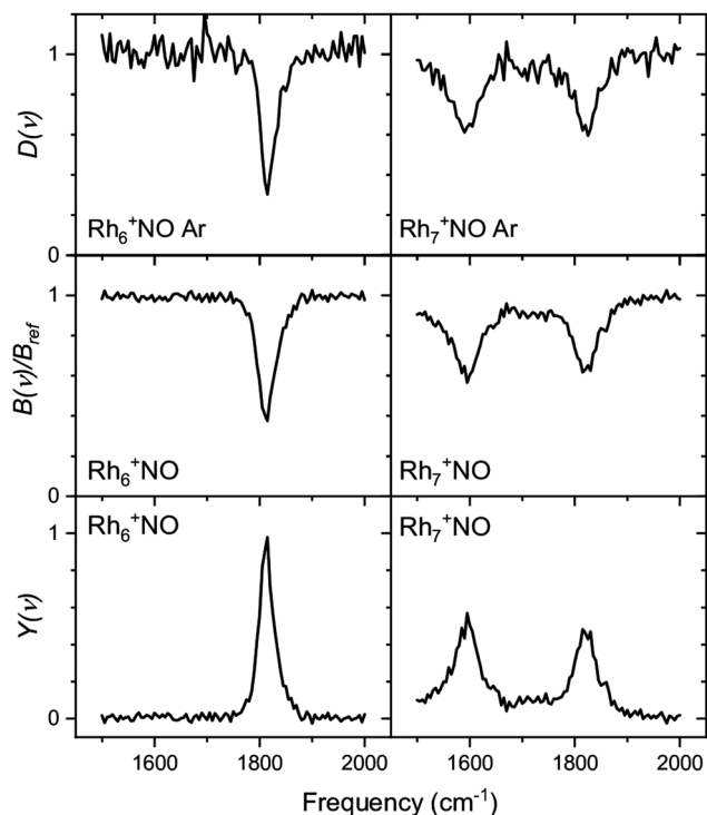
Fig. 2 Comparison between depletion D(\nu) for Rh_n^+NO -Ar (top rows), branching ratio depletion B(\nu)/B_{ref} (middle row), and photofragmentation yield Y_B(\nu) for Rh_n^+NO -Ar m ( m = 1-3 ) for n = 6 and 7 . Data from ref. 91.
