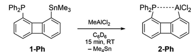
Scheme 2 Al-Sn exchange starting from 1-Ph and MeAlCl 2 to give 2-Ph .
