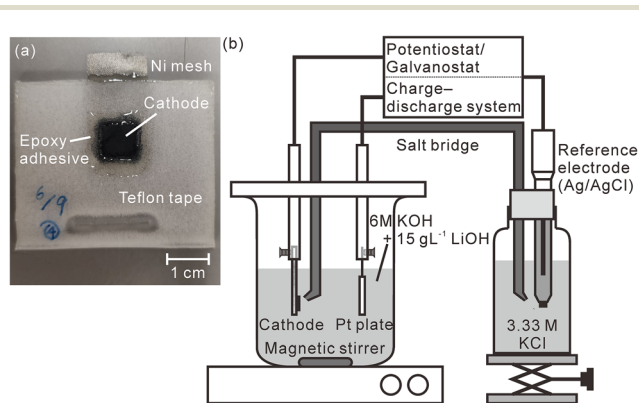
Fig. 1 (a) Photograph of the model cathode and (b) schematic illustration of the charge–discharge test apparatus. The measured area is enclosed within the dotted line in Fig. 1(a).
