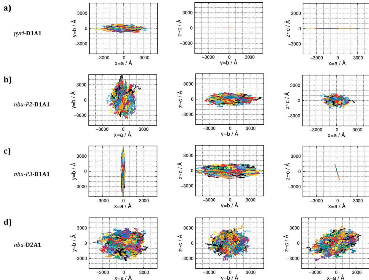
Fig. 7 Plot of 1000 kMC trajectories (each consisting of 10^5 steps) for each D1A1 and D2A1 class (from top to bottom: pyr1 -, nbu-P2 -, nbu-P3 - D1A1 and nbu - D2A1 ). Trajectories are reported for the three Cartesian planes, namely yx , zy and zx (crystallographic axes are reported as well).
