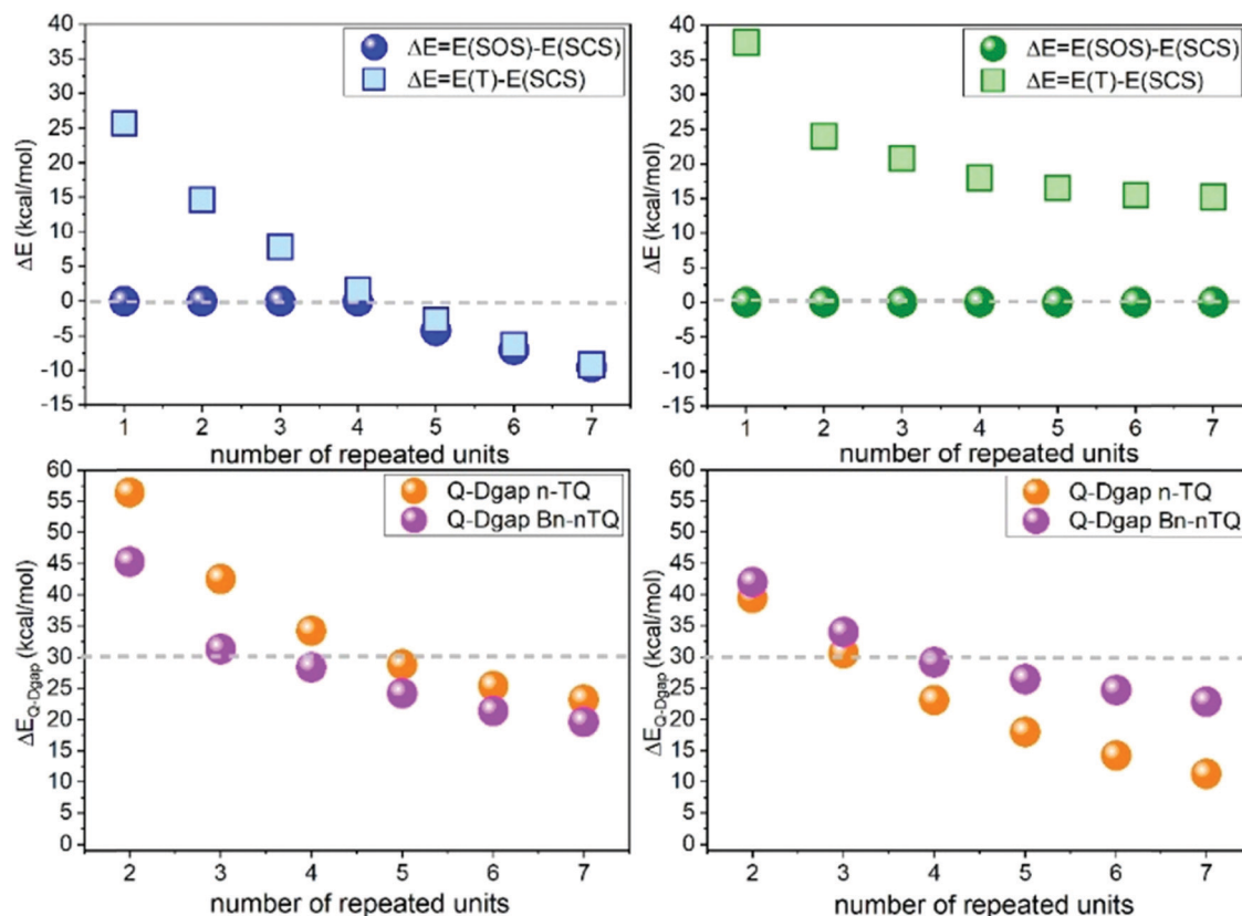
Fig. 8 Top: DFT/(U)B3LYP calculations of the energy differences ( \Delta E ) between the singlet closed (SCS) or open-shell (SOS) ground electronic states and the first excited state triplets (T) in the nTQ (left) and Bn-nTQ (right) series. Bottom: DFT/UB3LYP calculations of the energy differences between the ground electronic state doublet (D) and first quarter excited state (Q) of the radical anions (left) and cations (right) of the same series.
