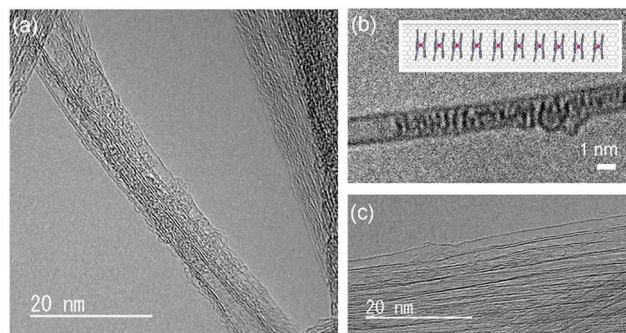
Fig. 2 Structural characterization of \text{TbPc}_2@SWCNT . Conventional bright field and phase contrast TEM images of \text{TbPc}_2 encapsulated in SWCNTs. (a) \text{TbPc}_2 was confirmed to be inside SWCNTs. Tb was detected by using EDX (see Fig. S3, ESI † ). (b) \text{TbPc}_2 were partially stacked one-dimensionally in SWCNTs. (c) Empty SWCNT.
