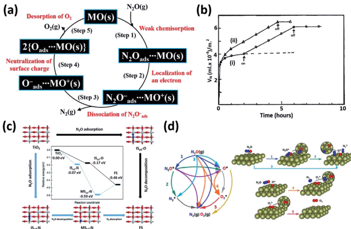
Fig. 12 (a) Mechanism of the conversion of N_2O to N_2 and O_2 over a metal oxide surface. (b) Time-dependent production of N_2 ( V_N ) from N_2O (10 Torr) over an activated ZnO surface at 20 °C under (i) dark and light on/off conditions indicated by arrows and (ii) continuous illumination. Reprinted with permission from ref. 152. Copyright© 1971, American Chemical Society. (c) Relative energy diagram for the photocatalytic decomposition of N_2O on perfect anatase (001) facets. Reprinted with permission from ref. 173. Copyright© 2018, Royal Society of Chemistry. (d) Reaction diagram for the conversion of N_2O to various adsorption and decomposition products ( N_2O^* , N_2^* , O^* , O_2^* , N_2(g) and O_2(g) ); * designates adsorbed species. (1–3) Dissociative adsorption of N_2O on Ir(111), (4) formation of surface peroxides, and (5) O_2 desorption from Ir(111). Reprinted with permission from ref. 177. Copyright© 2019, American Chemical Society.
