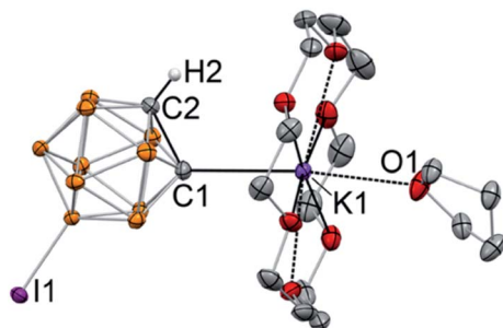
Fig. 2 Displacement ellipsoid plot (50% probability) of [K(18-crown-6)(THF)][C 2 B 10 H 10 I] (3). Hydrogen atoms except H2 have been omitted for clarity. Selected bond distances (Å): K1–C1 = 2.978(1), C1–C2 = 1.682(1).
